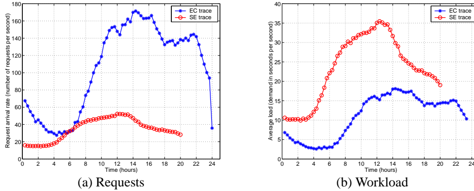
Fig. 4. Trace Request Arrivals and Workload
