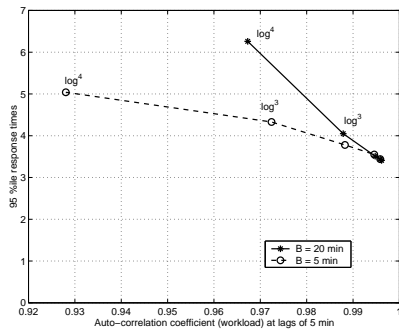
Fig. 9. Impact of Autocorrelation
