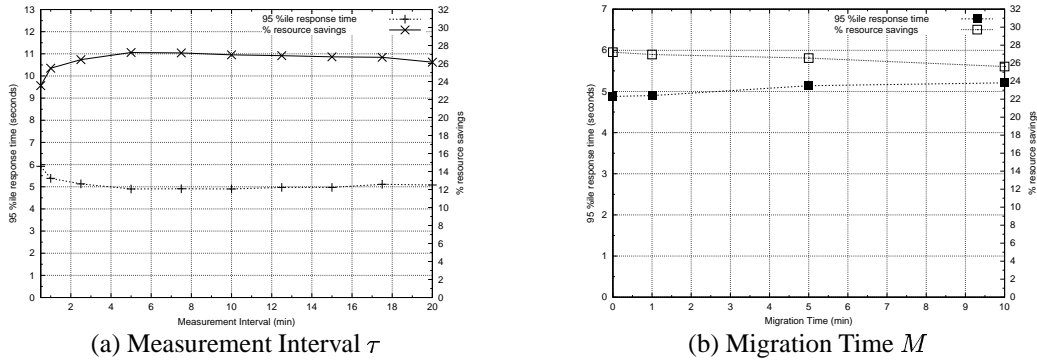
Fig. 6. Impact of \tau and M on QoS and Resource Savings
