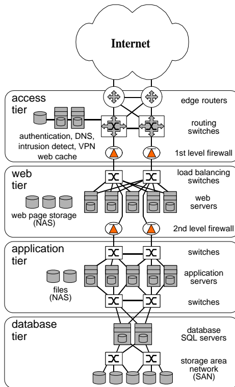
Fig. 1. IDC Four Tier Architecture
