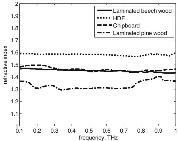
Fig. 3 Refractive indices of wood samples: laminated beech wood, HDF, chipboard, laminated pine wood.
