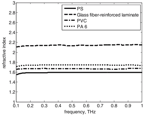
Fig. 9 Refractive indices of plastic samples: polystyrene (PS), glass fiber-reinforced laminate, polyvinyl chloride (PVC), polyamide 6 (PA 6).
