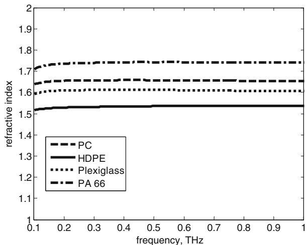
Fig. 10 Refractive indices of plastic samples: polycarbonate (PC), high-density polyethylene (HDPE), clear cast acrylic (Plexiglass), polyamide 66 (PA 66).
