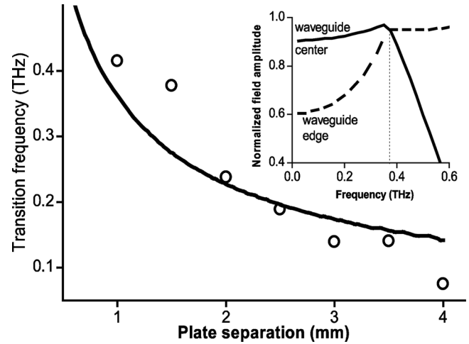
FIG. 3. The transition frequency as a function of the plate separation b . The black circles are the experimental results and the solid line is the calculated curve from the theoretical model described in the text. The inset shows two vertical cuts extracted from the data of Fig. 2(a), for b = 1.5 mm. The cross-over point of these two curves defines the transition frequency.
