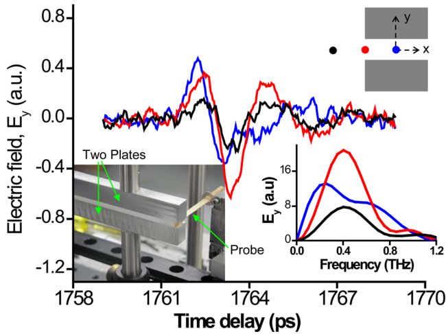
FIG. 1. (Color online) Signals measured inside (blue), at the edge (red), and outside (black) of the waveguide. These locations are illustrated by the cross-sectional view in the upper-right inset. The lower-right inset shows the corresponding spectra, which all have spectral bandwidths similar to that of the input THz pulse. These indicate that the scattering probe technique does not introduce any significant spectral distortion or bandwidth limitation on the measured signals. The left inset shows a photograph of the PPWG with the scattering probe inserted between the plates. The plate-width along the x direction is 10 mm.
