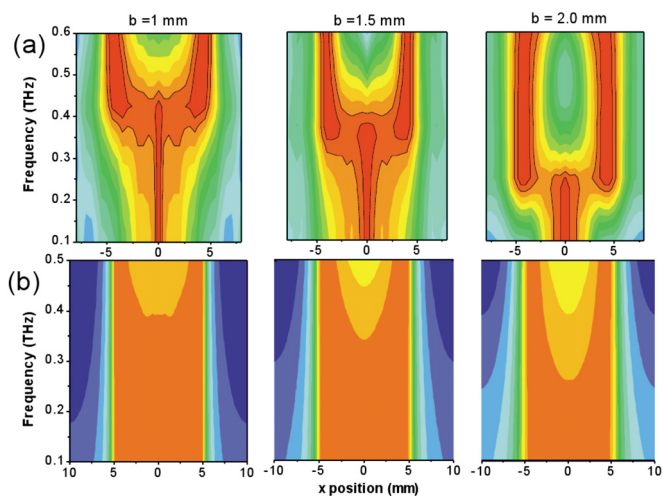
FIG. 2. (Color online) Contour plots of the normalized cross-sectional electric field distribution based on (a) experimental data and (b) numerical simulations using the finite element method. The horizontal axis gives the location of the measurement and the vertical axis gives the frequency. The waveguide extends from x = -5 to 5 mm. Each row of these figures has been normalized to unity, in order to remove the spectral dependence of the input pulse and emphasize the frequency-dependent mode transition. Results for three different values of the plate separation b are shown.
