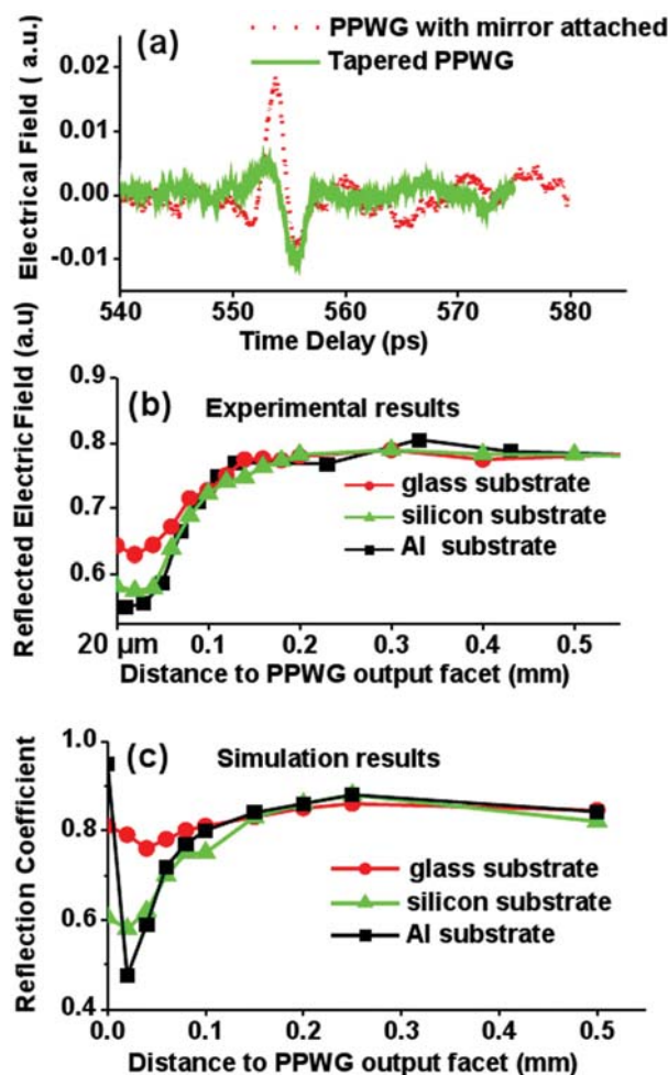
FIG. 2. (Color online) (a) Time-domain reflections from an untapered PPWG of plate spacing 2 mm with attached mirror and from a PPWG with tapered plate spacing, from 2 mm to 200\ \mu\text{m} . (b) Measured reflected electric field as a function of sample distance to the waveguide output facet, for glass, silicon, and aluminum (flat) samples. (c) Simulated reflection coefficients corresponding to the configurations in (b).
