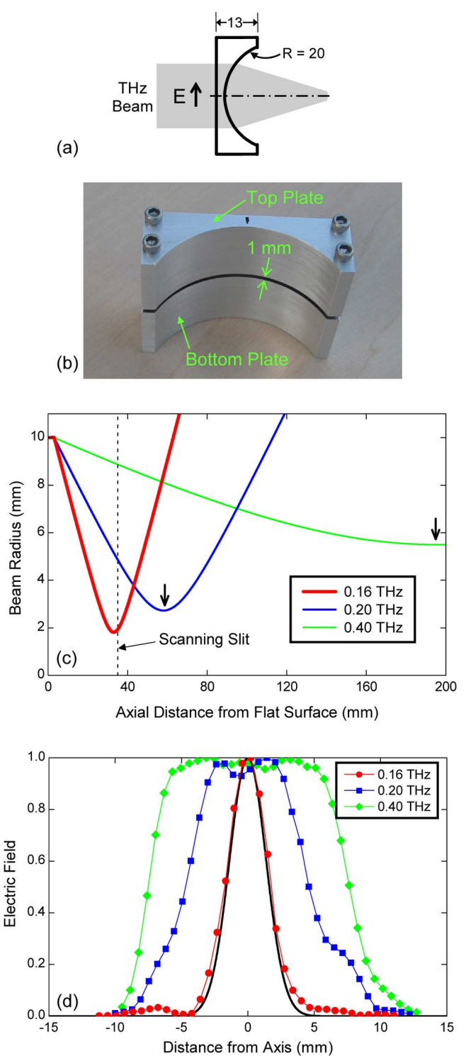
Fig. 4. (a) Schematic of the PPWG-lens. The width of the input face is 40 mm. Dimensions in millimeters. (b) Photograph of the fabricated device indicating the 1-mm gap between the two plates. (c) Gaussian beam calculation of the evolution of the output-beam radius for 0.16 THz (red in online version), 0.20 THz (blue in online version), and 0.40 THz (green in online version). The dashed line (35 mm away from the flat input surface) indicates the path of the slit. The vertical arrows indicate the foci. (d) Derived experimental electric field profiles at the 35-mm transverse plane. The solid black curve is the theoretical Gaussian profile for 0.16 THz.
