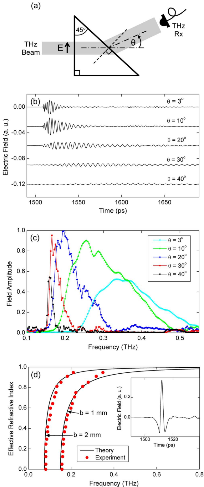
Fig. 1. (a) Schematic of the PPWG-prism. The width of the input face is 38.1 mm. (b) Terahertz signals detected at various Rx (angular) positions. (c) Corresponding amplitude spectra. (d) Comparison of the experimental and theoretical effective refractive index. The inset gives the input signal to the prism, which has frequency components varying from close to dc to about 1 THz.
