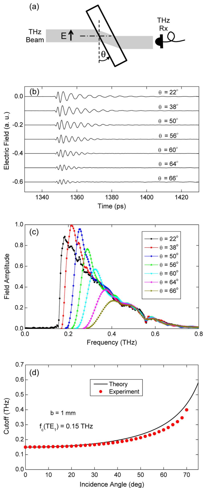
Fig. 2. (a) Schematic for the total-internal-reflection demonstration. The width of the input face is 31.8 mm. (b) Terahertz signals detected while rotating the PPWG with respect to the incident beam. (c) Corresponding amplitude spectra. (d) Comparison of the experimental and theoretical cutoff.
