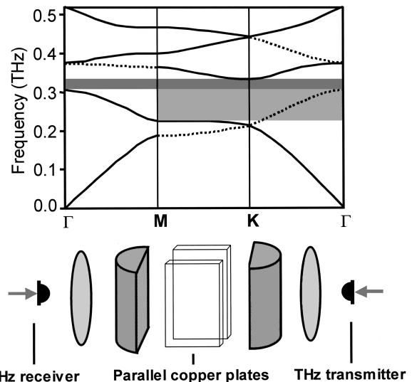
Fig. 1. Top, 2D band structure (TM polarization) of the photonic crystal used in these measurements. This band structure is computed assuming an infinite slab thickness. 20 The shaded boxes indicate the full gap (darker) and the pseudogap (lighter), and the dashed bands are antisymmetric and therefore do not couple to the incident beam. Bottom, schematic of the experimental setup. The photonic crystal is placed within the copper waveguide for transmission measurements.
