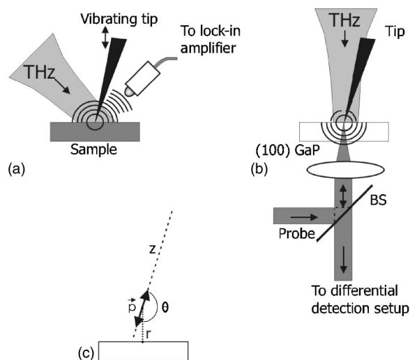
FIG. 1. (a) “Far-field” THz ANSOM setup. The THz pulse is detected in the far-field while the tip is vibrated. (b) “Near-field” THz ANSOM setup. The THz pulse is detected in the near-field of the tip. (c) Angle and coordinates of the oscillating dipole.
