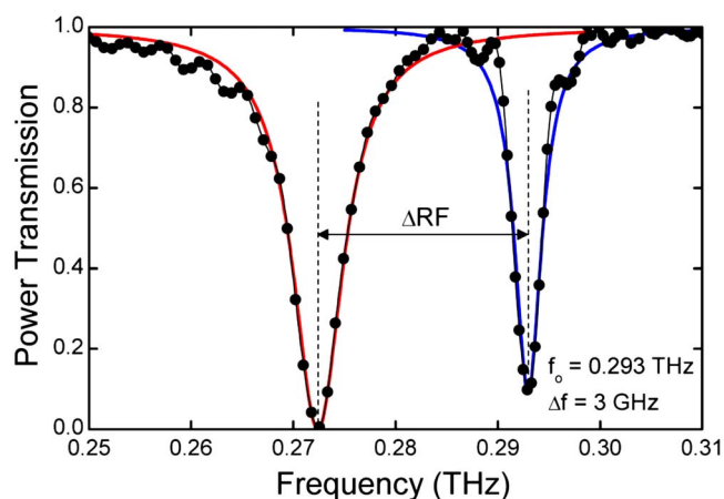
FIG. 4. (Color online) Power transmission (dots) in the vicinity of the resonance dips, derived by taking the square of the ratio, and the inverse-ratio, of the spectra in Fig. 3. These are fit to Lorentzian line shapes (blue and red solid curves). These fits indicate a resonant frequency of 0.293 THz and a linewidth of 3 GHz for the empty cavity, and a linewidth of 6 GHz and an extinction coefficient of 30 dB for the filled cavity. This result is used to derive the resonant-frequency shift ( \Delta RF ) for each of the different liquids studied.
