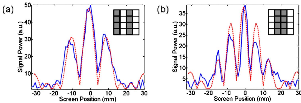
FIG. 4. (Color online) Measured (solid curves) differential fringe patterns produced by the transmission of the terahertz beam through the terahertz SLM in two double-slit configurations, compared with analytical calculations (dashed curves). The insets show the “on” and “off” configurations of the 16 pixels, with zero bias on the gray pixels, and the white pixels modulated with a 3 kHz square signal alternating between 0 and 14 V.
