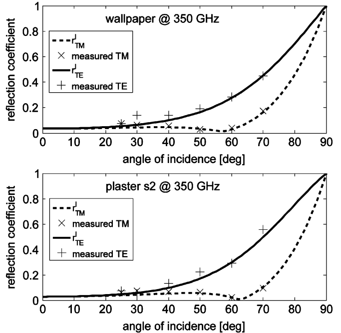
Fig. 11. Calculated magnitude of modified reflection coefficients r'_{TE} and r'_{TM} and direct reflection measurements of wallpaper and plaster sample 2 for angles of incidence between 0° and 90° at a frequency of 350 GHz for TE and TM polarized waves.
