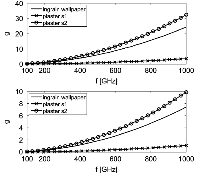
Fig. 4. Calculated parameter g for the three samples for angles of incidence of 25^\circ (top) and 60^\circ (bottom).
