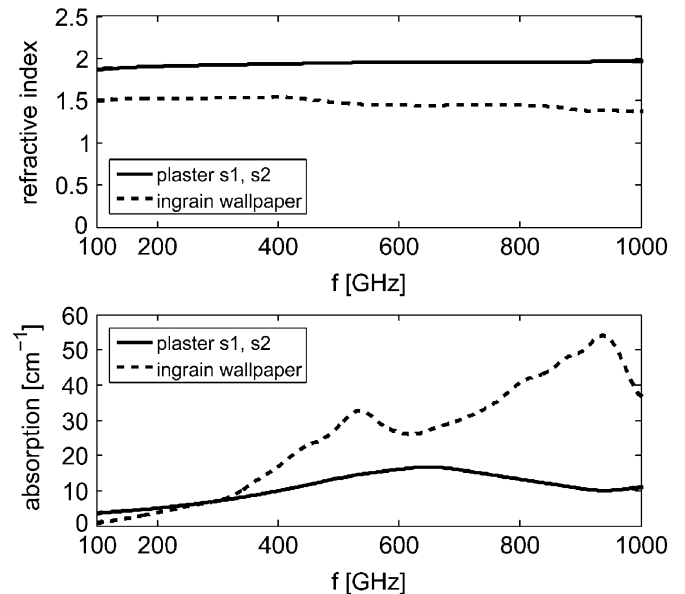
Fig. 7. Measurements of refractive index (top) and absorption coefficient (bottom) of the investigated samples in transmission geometry.
