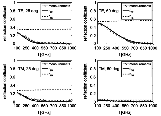
Fig. 10. Calculated magnitude of reflection coefficients r_{TE} and r_{TM} and of modified reflection coefficients r'_{TE} and r'_{TM} and direct reflection measurements of plaster sample 2 in the frequency range from 100 to 1000 GHz for two angles of incidence of TE and TM polarized waves: 25°, 60°.
